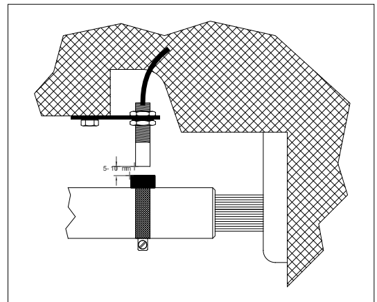
Rys. 5-1 Sensor X na wale kardana
